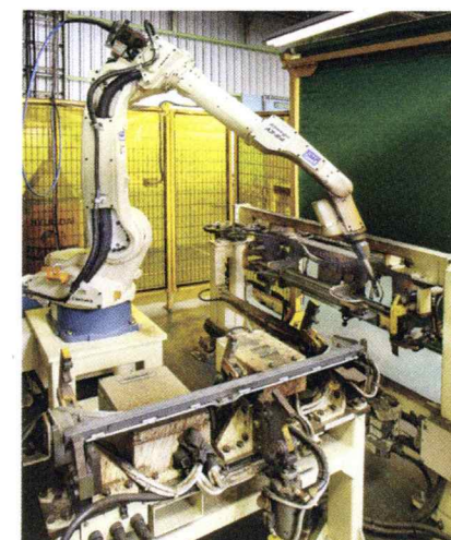
OEW溶接設備
